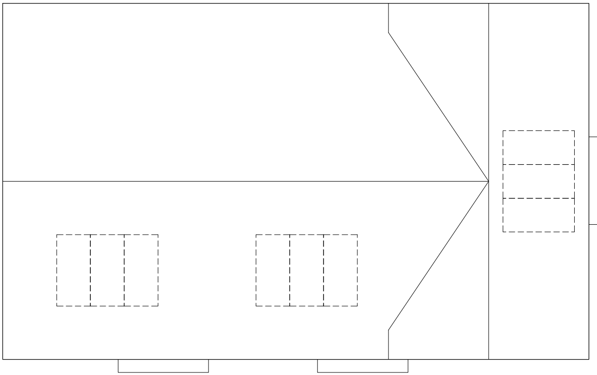
ROOF PLAN
