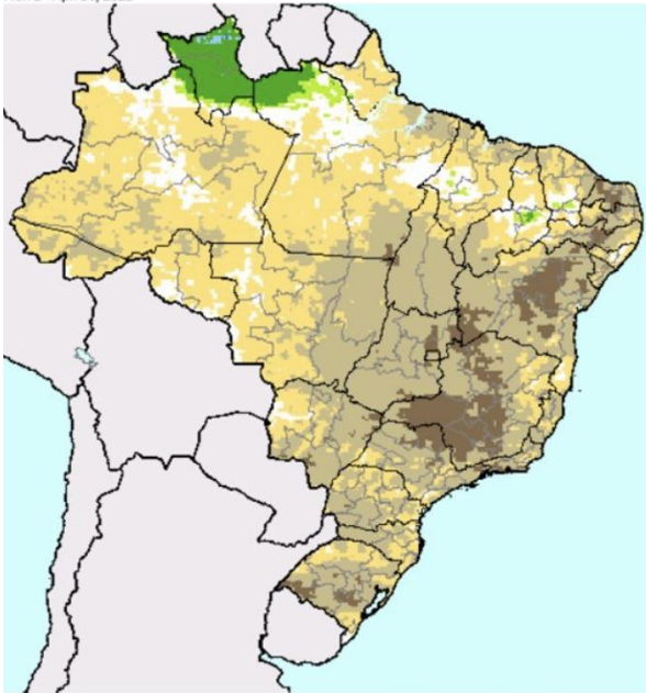
Seasonal Percent of Normal Precipitation (USAF 557th WW) Mar. 1 - Apr. 10, 2021
