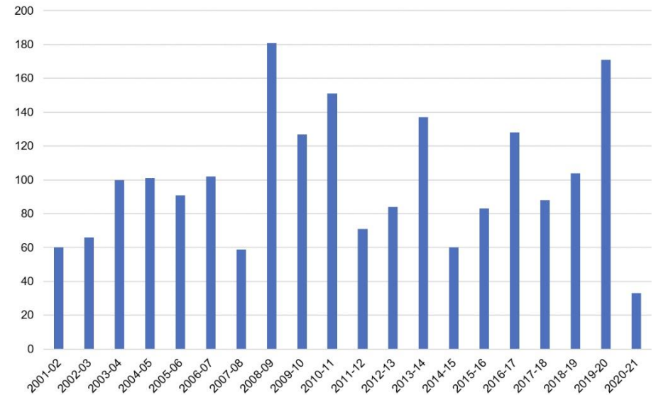
North Dakota Precipitation: % of normal, Sept. – March
