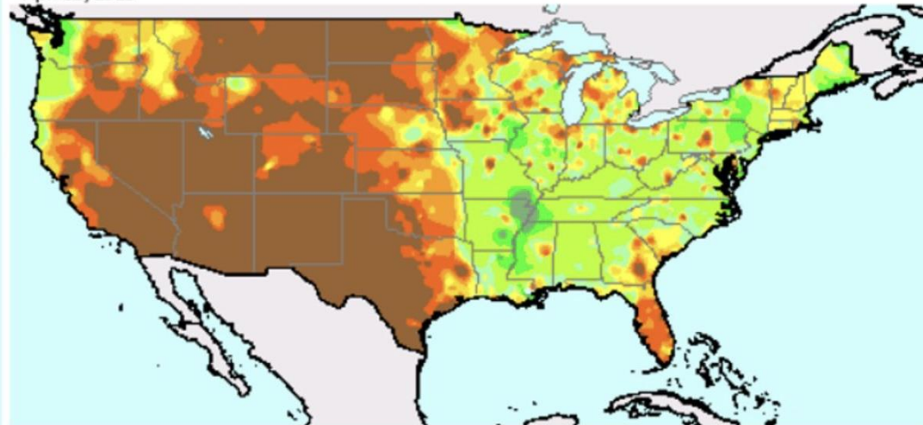
Subsurface Soil Moisture (WMO) Apr. 11, 2021
