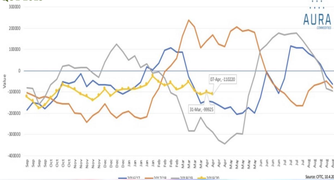
CFTC Corn Futures - Managed Money Net Positions April 7th, 2020 Week End
