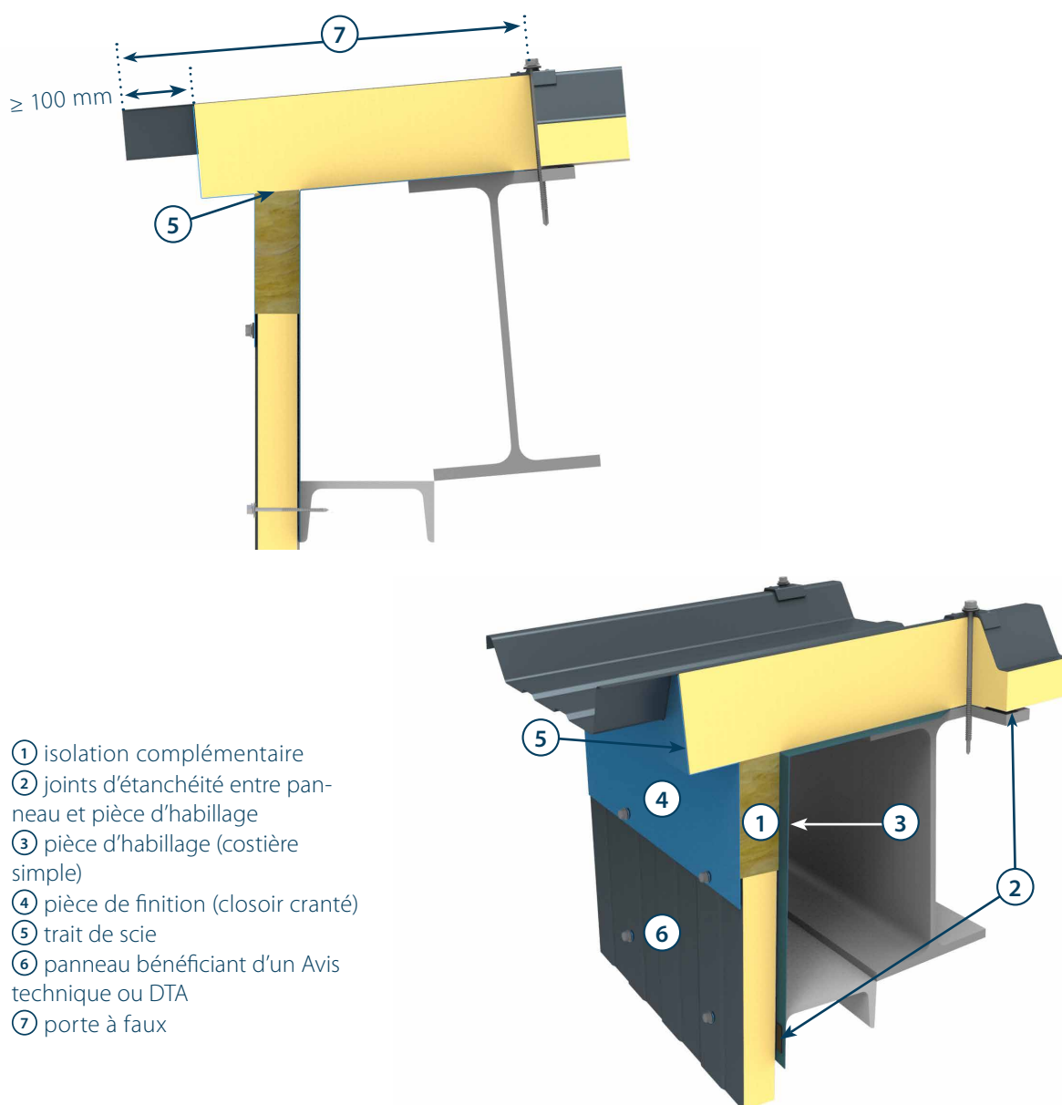
Figure 22 : Egot simple
