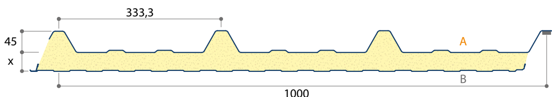
Figure 1 : Panneau JI Roof 1000 IPN
