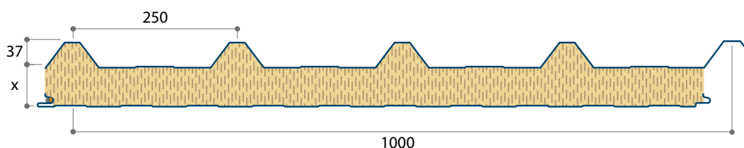
Figure 30 : Panneau JI Vulcasteel Roof
