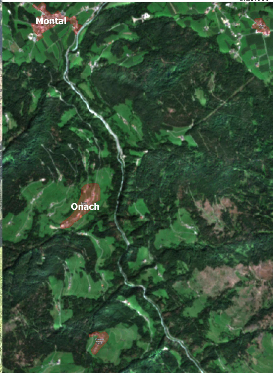
SENTINEL 2 - Mosaik 2021
