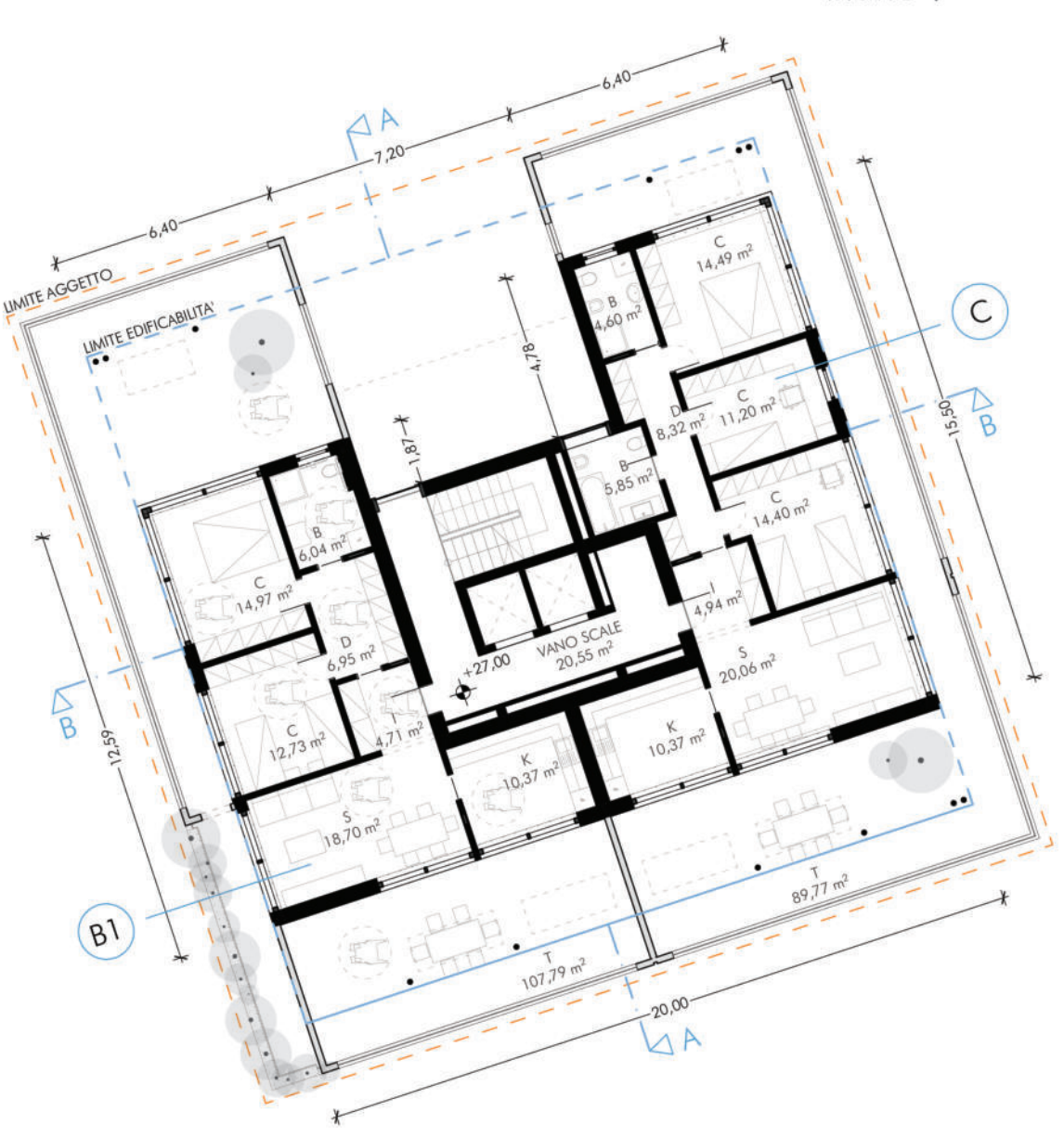
Piano 9°
