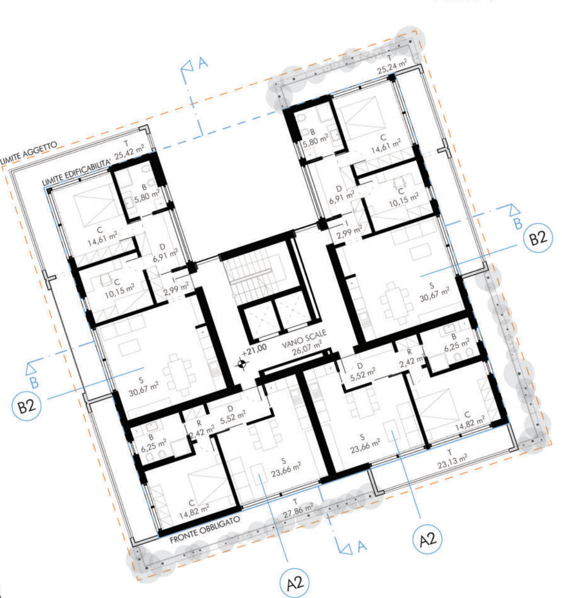
Piano 7°
