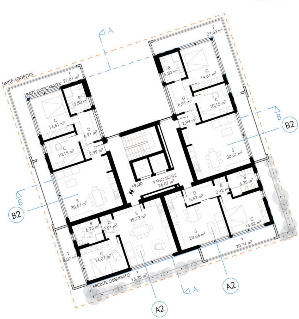
Piano 3°
