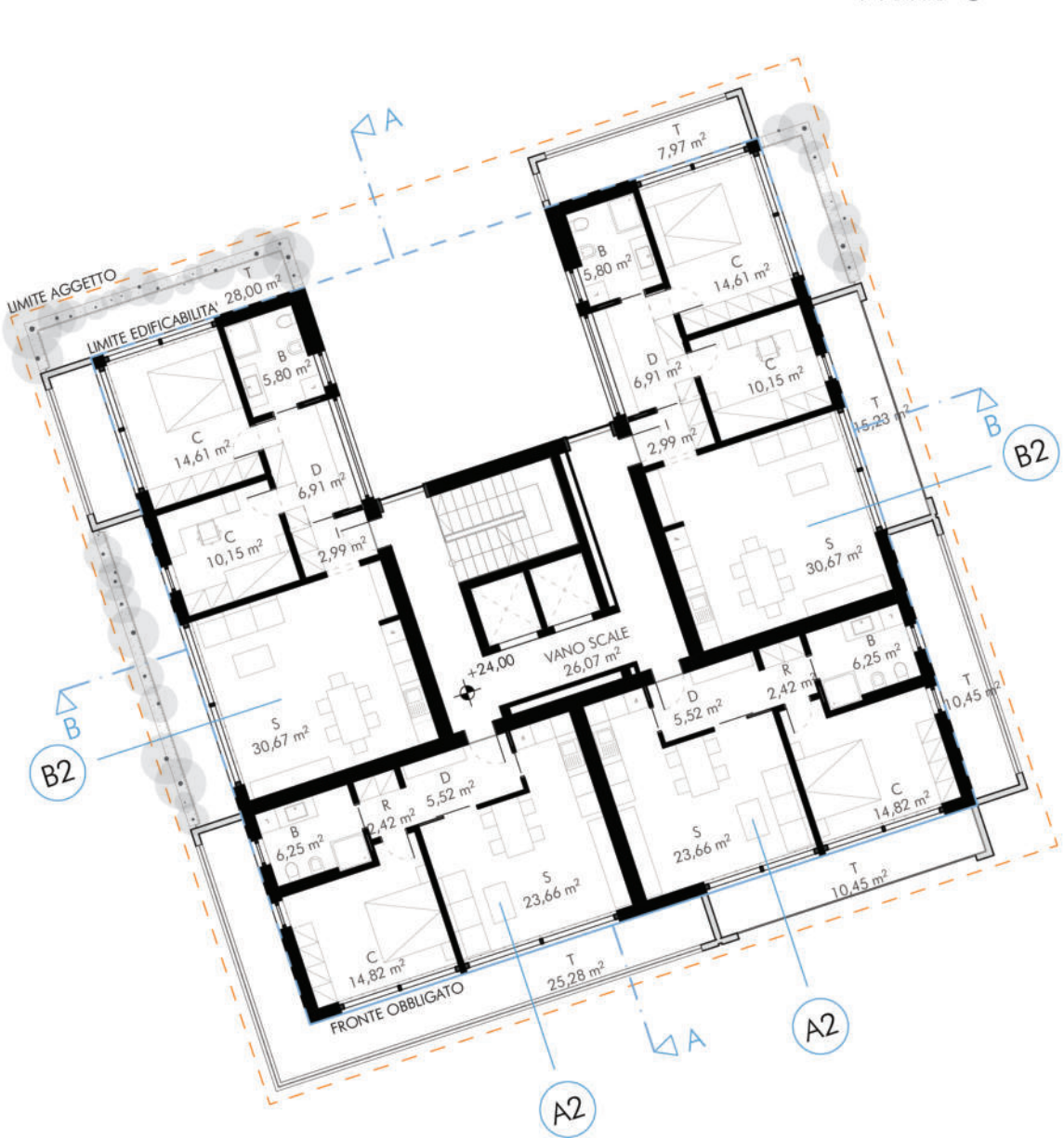
Piano 8°
