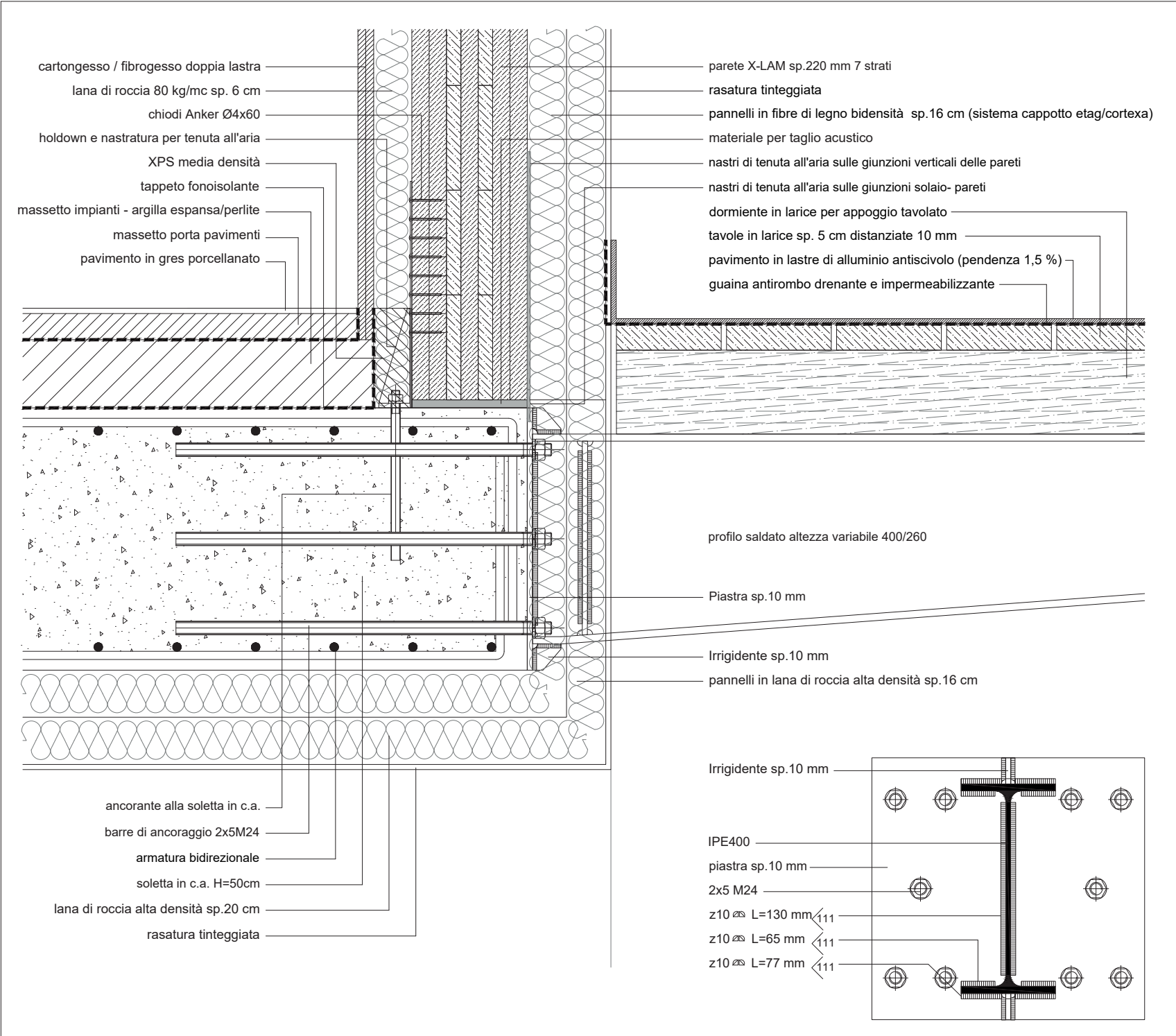
nodo soletta in C.A. parete esterna in X-LAM
