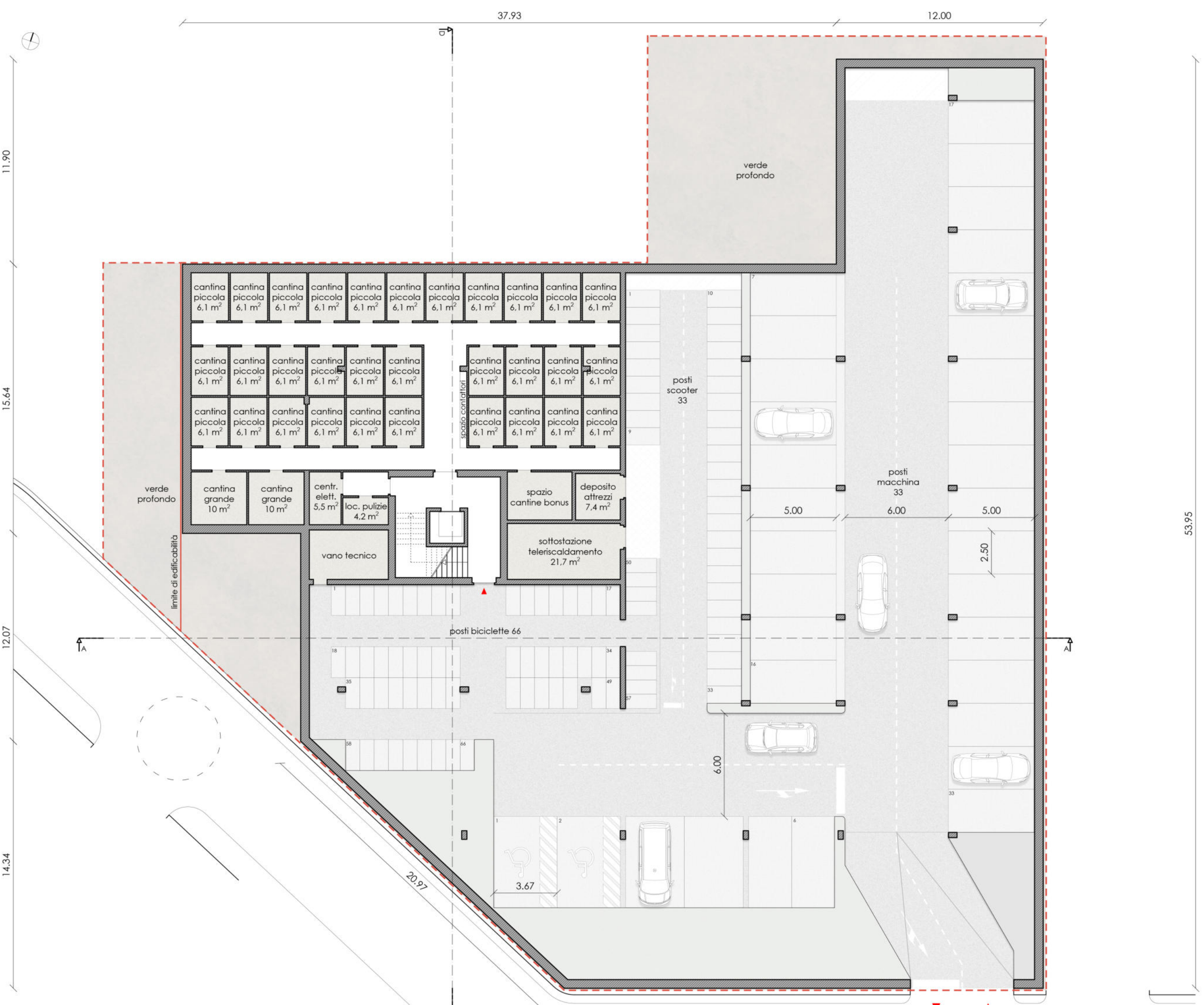
PIANO GARAGE SCALA 1:200
