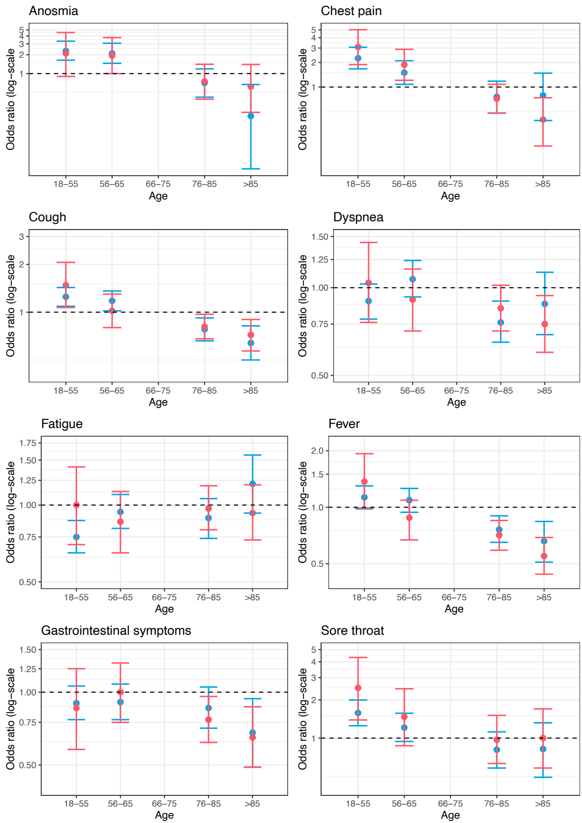
Figure S3: Complaints at presentation stratified by age and prior history of cardiac disease. Red = patients with pre-existing cardiac disease, blue = patients without pre-existing cardiac disease.
