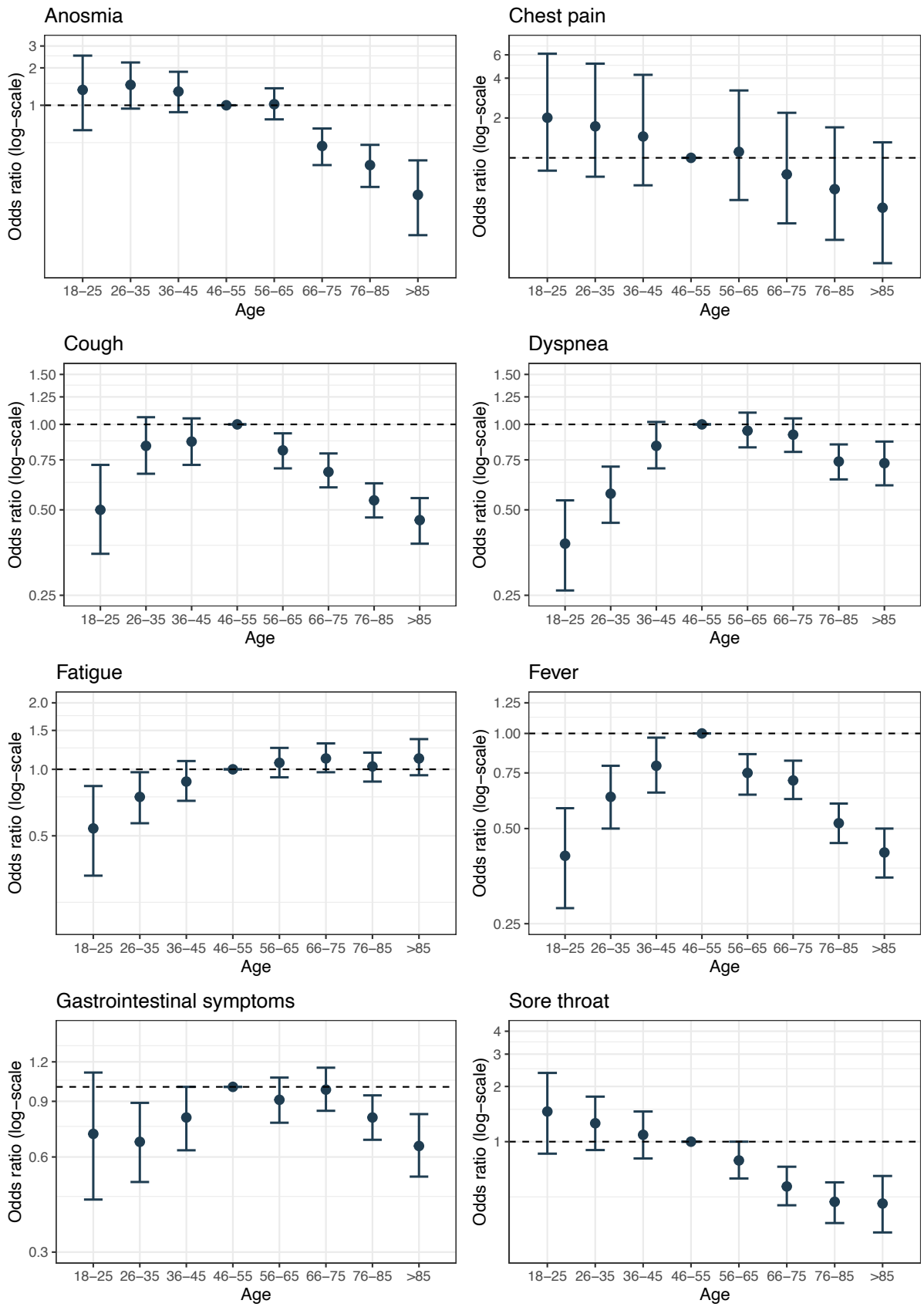
Figure S2: Complaints at presentation stratified by age.
