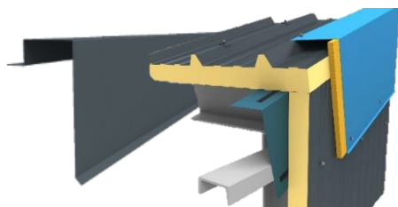
Flashings
