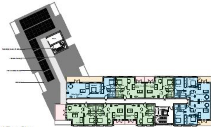
Proposed Third Floor Plan
