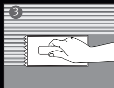
3 Apply second pass of Basecoat to enclose Stormshield Mesh Cloth and to a total thickness of 10mm; finish with a horizontal keyed finish
