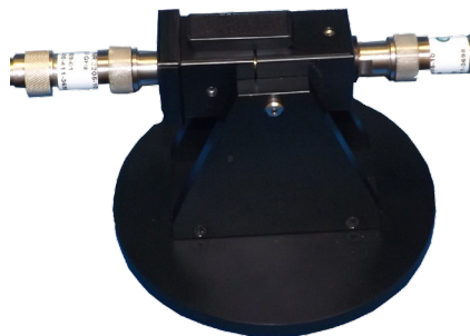
Fig 2. Test fixture for SE measurements at f = 1.5 - 10 \text{ GHz} .
