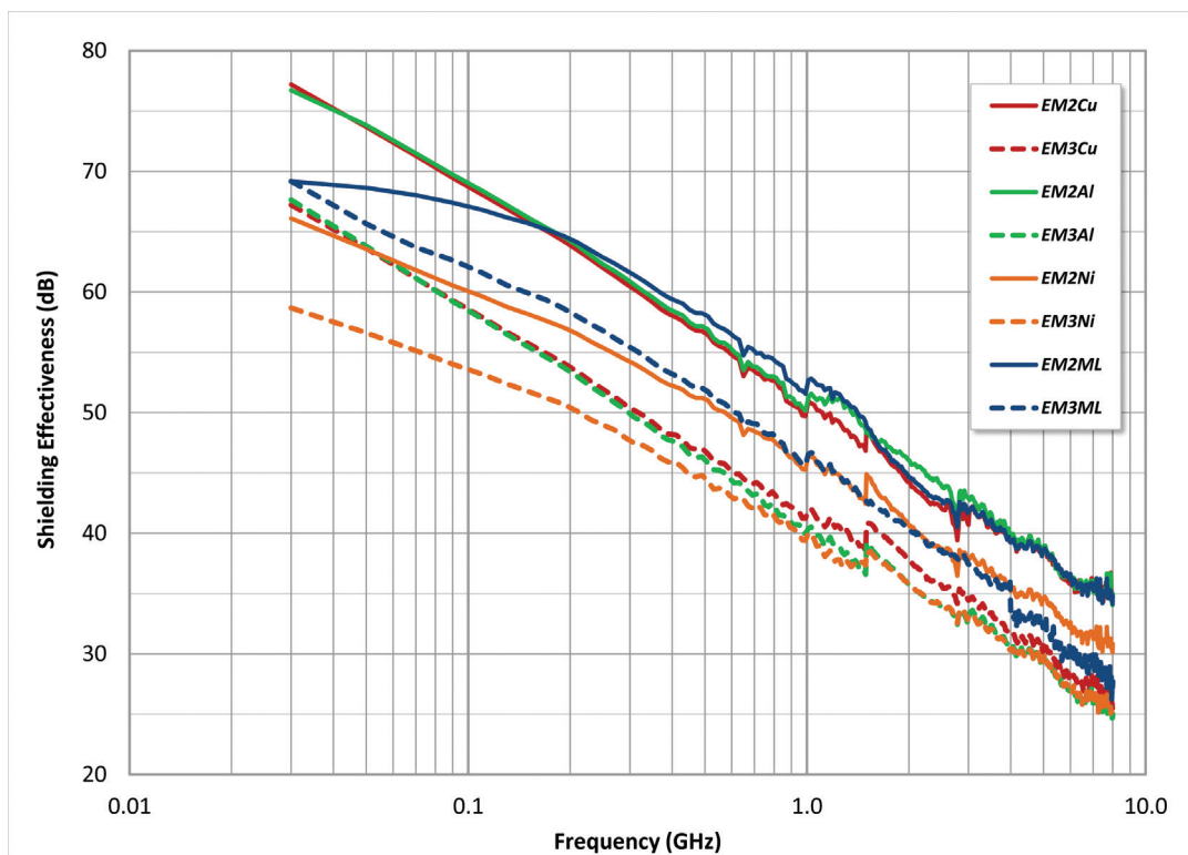
Fig 7. Measured shielding effectiveness (SE) of MicroGrid EM standard foils for EMI shielding.
