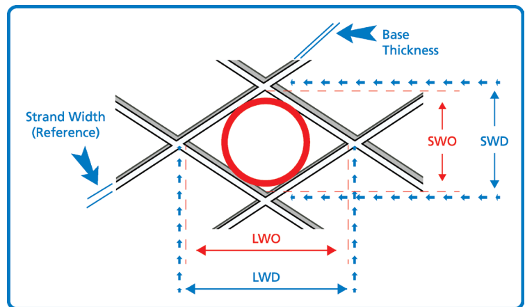
Fig 4. Dimensions of expanded metal foils
